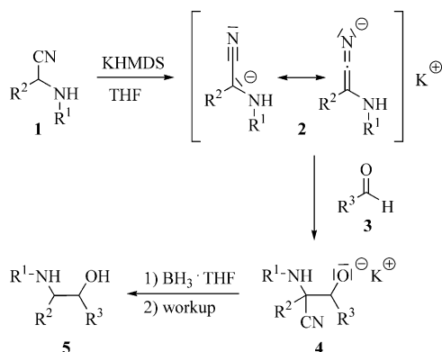
Scheme 1. Mechanism of the reaction of \alpha -amino nitriles to form amino alcohols.
