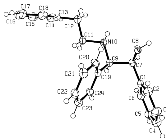
Figure 1. Crystal structure of anti - 5h at 193 K (ORTEP). Thermal ellipsoids are drawn at the 50% probability level.
