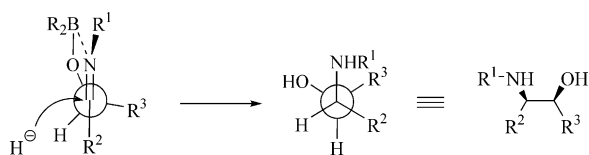
Scheme 2. Chelate model for the reduction step.
